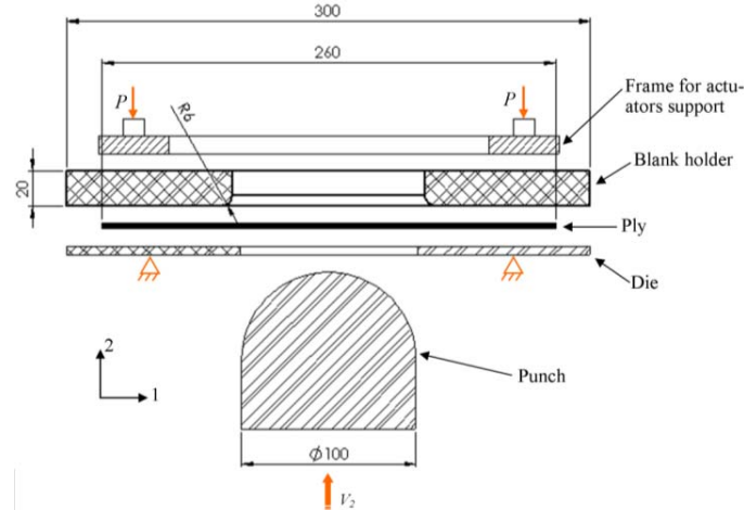
Fig 1: Forming machine scheme with characteristic dimensions. All dimensions are in mm.
