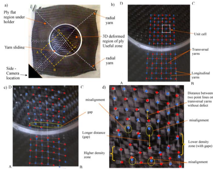
Fig 4: intra-ply yarn sliding on ply-45 after preforming with 0.075 MPa operating pressure. Top view (a), zoomed portion (ABCD) before preforming (b), after preforming (c) and zoom on the defect zone after removal of the blank-holder plate (d).
