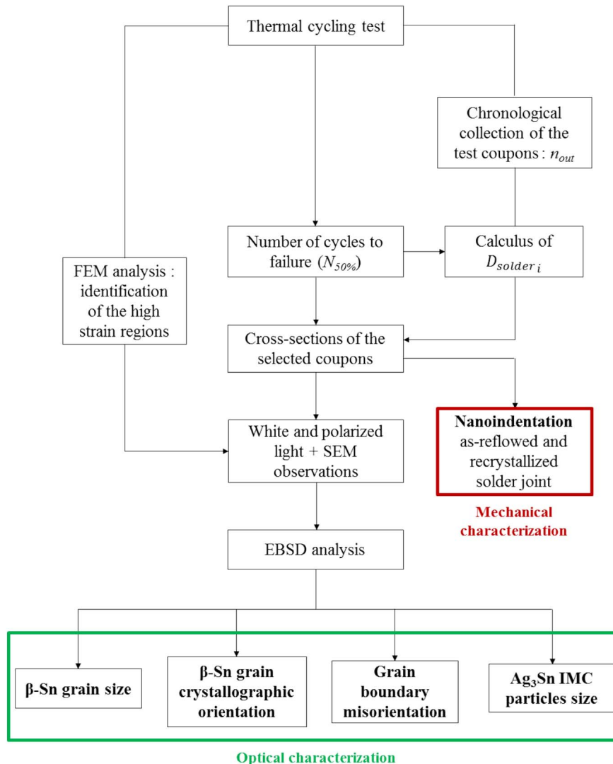
Fig. 3. SAC305 microstructural evolution investigation approach.
