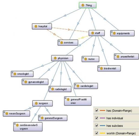
Fig. 4: A snapshot of hospital ontology created by OntoGraf in Protégé 4.3 (Staff level)
