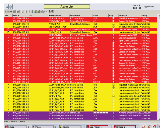
Figure 1. The flood alarm display screen
