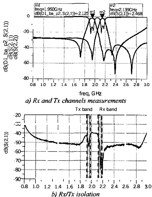
Figure 9. Duplexer measurements.
