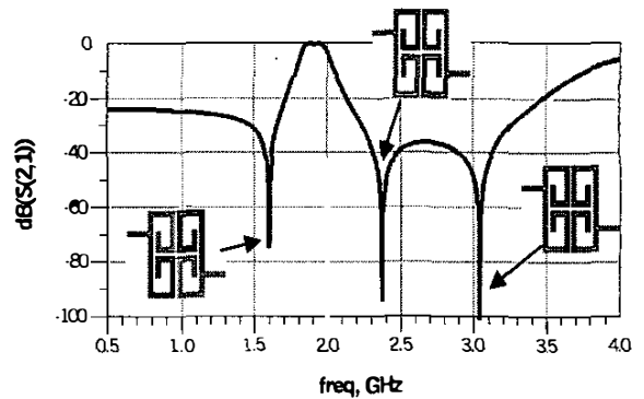
Figure 3. Transmission zero frequencies and related lengths.
