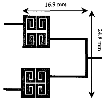
Figure 8. Duplexer layout
