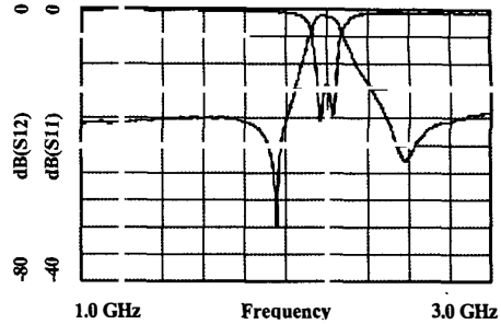
Fig.11. Measurements
