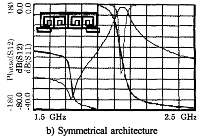
Fig. 6. S parameter responses and transmission phase variation of a “two resonators” structure.
