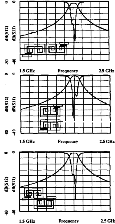
Fig. 4. No-transmission zero topologies by means of two unsymmetrical coupled resonators
