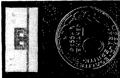
Fig. 3. Photography of the single resonator structure.
