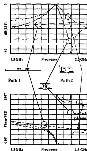
Fig. 1. Single resonator with a transmission zero : Principles
