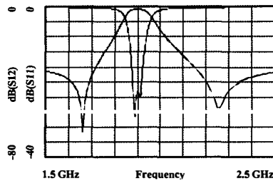
Fig. 9. Simulation response of the 2 zeros structure.
