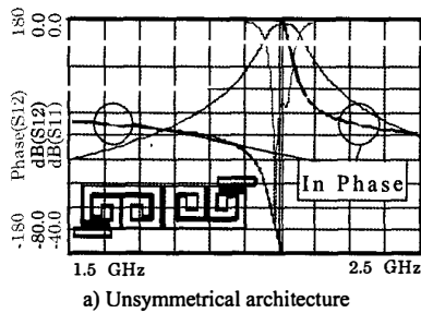
a) Unsymmetrical architecture
