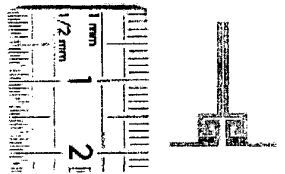
Fig. 10 Photography of the realized two resonators structure.
