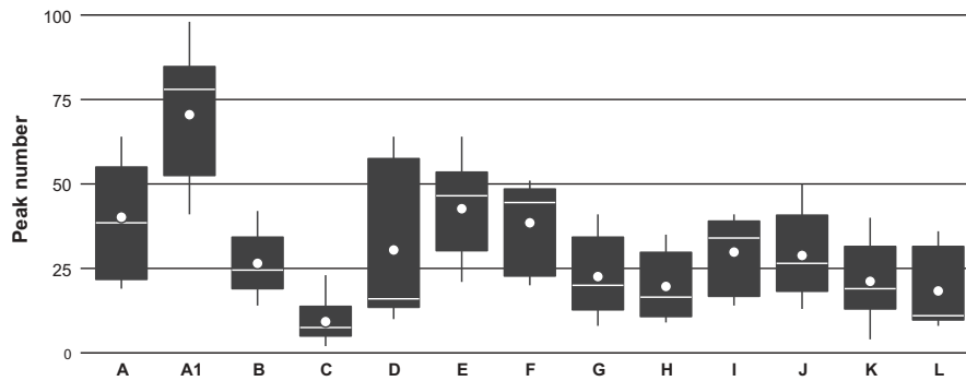
Figure 3. Box plots of the number of peaks detected with different extraction protocols used (A–L; see Table 2). The data are aggregates of three isolates: Lemonniera terrestris LETE 184-1681, Neonectria lugdunensis NELU 130-1656, and Tricladium splendens TRSP 180-1649. White line: median; white dot: mean; lower limit of the black box: 25th percentile; upper limit: 75th percentile; error bars: values within 1.5 interquartile range. Data of the individual isolates are presented in SUPPLEMENTARY FIG. 1.
