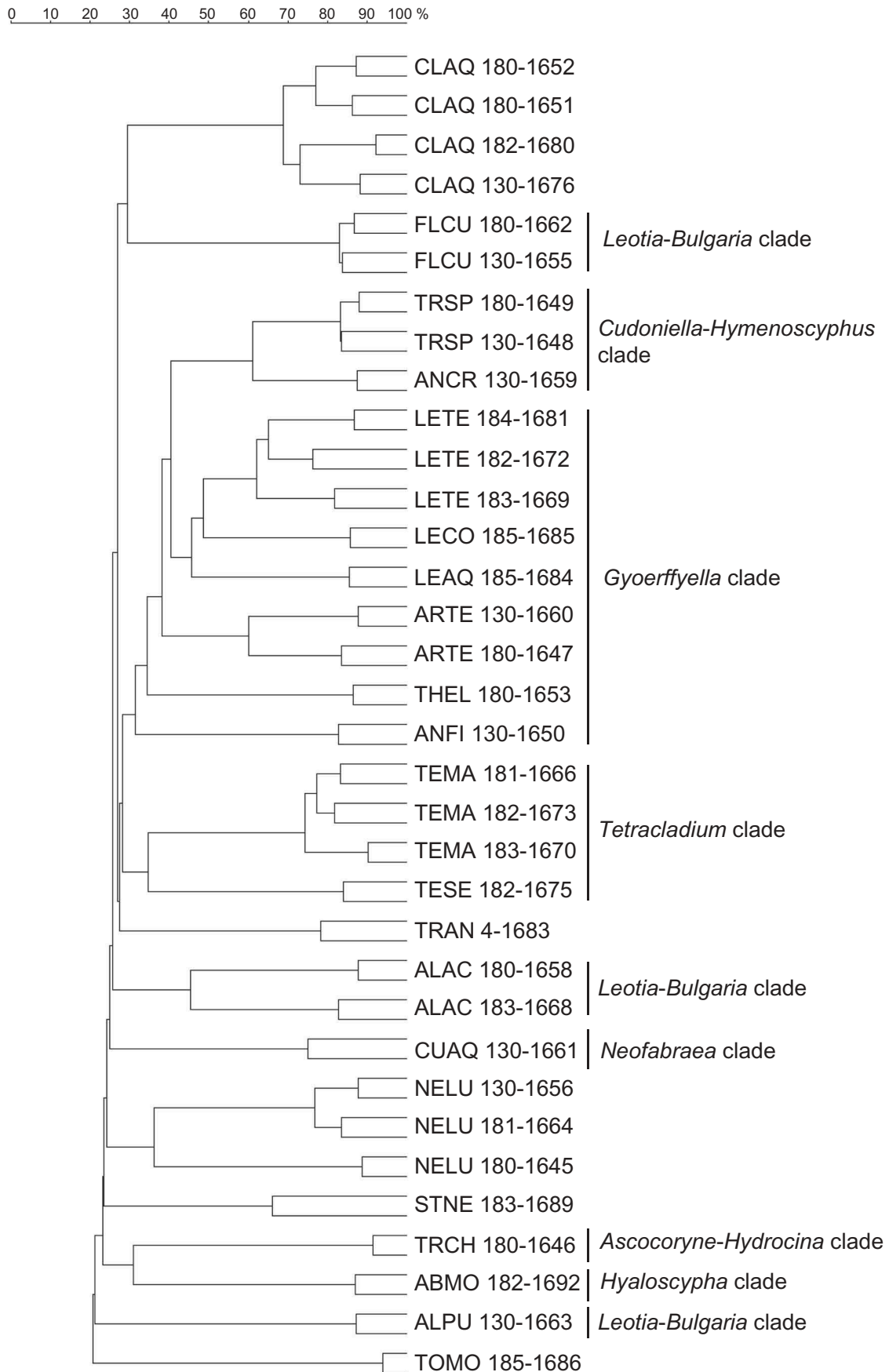
Figure 4. Dendrogram (single linkage agglomerative clustering) based on the MALDI-TOF MS analysis of the aquatic hyphomycete isolates (using protocols A and A1, see details in text and in Table 2 ). Two MALDI-TOF mass spectra per isolate are shown to represent analytical variability; mass range: 3000–20 000 m/z , averaged smoothing (width: 50 channels) and baseline subtracted (width: 500 channels), tolerance: 0.08%.
