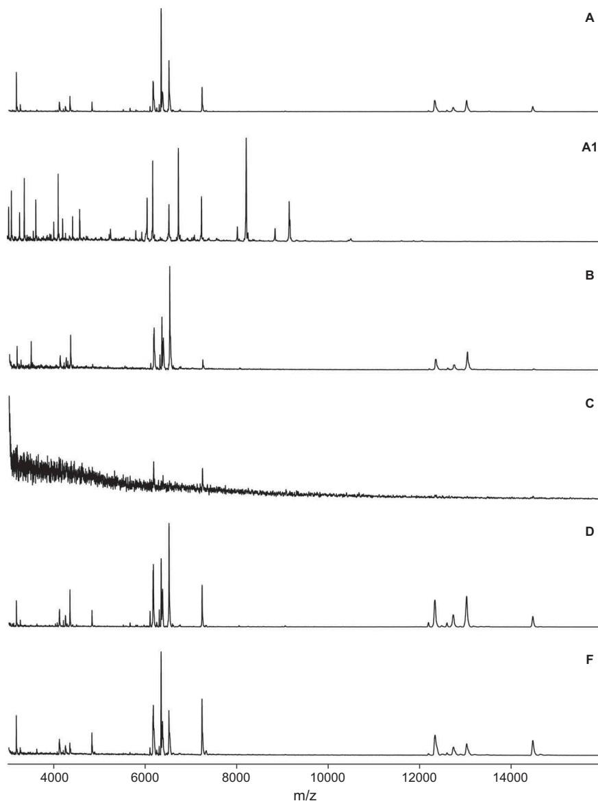
Figure 2. MALDI-TOF mass spectra of N. lugdunensis (NELU 130-1656) obtained using six different protocols (A, A1, B, C, D, F; for details, see Table 2). Relative intensities shown; averaged smoothing (width: 50 channels) and baseline subtracted (width: 500 channels), tolerance: 0.08%.
