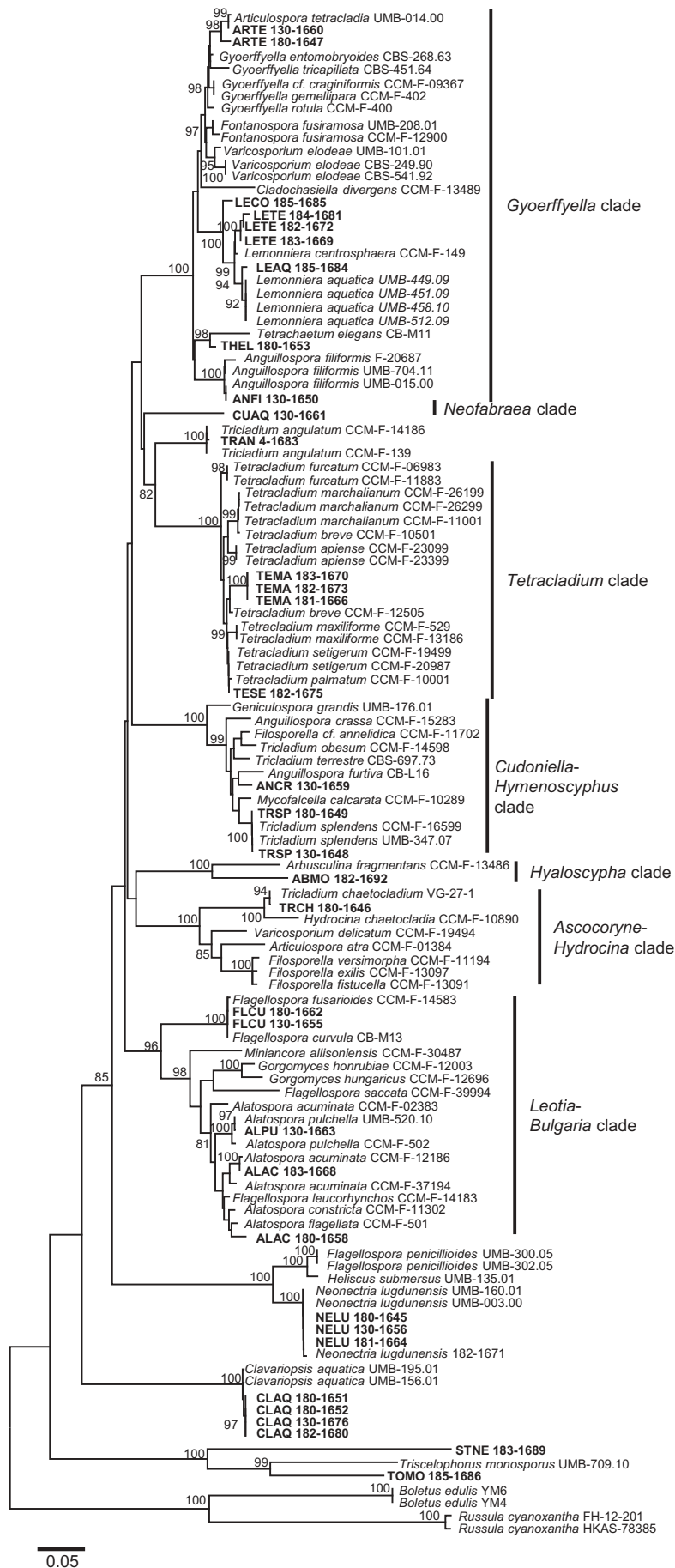
Figure 1. Phylogenetic tree based on ITS sequences of aquatic hyphomycetes. Neighbor-joining method using the Kimura two-parameter distances; bootstrap support of 80% or greater from 1000 replicates is shown in the internal nodes of the branches. Isolates used for this study are highlighted in bold.
