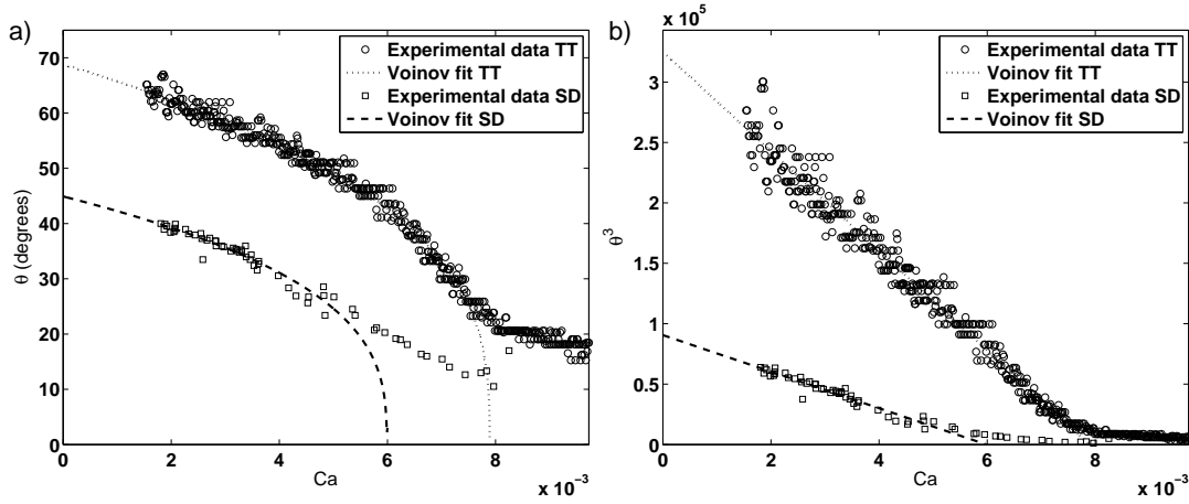
Fig. 4: Dynamic contact angle \theta as a function of the capillary number (normalized contact line velocity). The circles and squares represent the data obtained from the turntable setup (TT) and sliding droplet experiment (SD), respectively. The dashed lines represent the fit based on Cox-Voinov relation (1).
