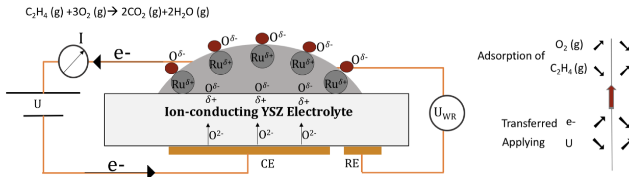
Figure 1: A schematic representation of ruthenium electrode deposited on O^{2-} conducting YSZ solid electrolyte, showing the locations of the metal/electrolyte double layer [ O^{\delta-} \delta^+ ] and the effective double layer created at the metal/gas interface. All electrodes are under the same gaseous conditions. The potential-controlled ion migration (backspillover) and charge transfer affect the adsorption strength of electropositive ethylene and electronegative oxygen gas species (shown on the right).
