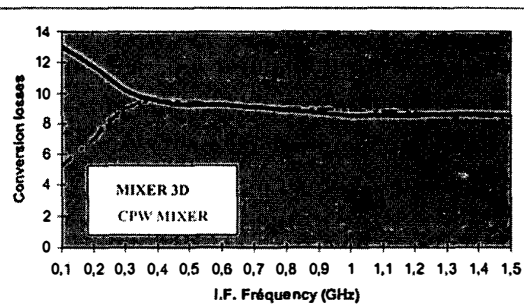
Fig. 9. Uniplanar/multitechnology mixer : Comparisons
