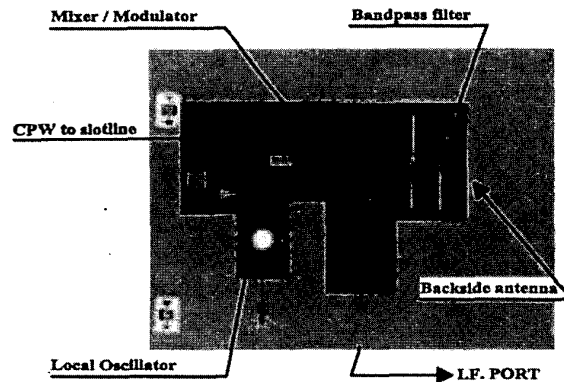
Fig. 8. Photography of the complete integrated module.
