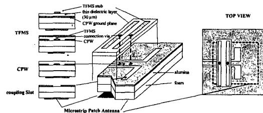
Fig. 1. Filter-antenna module on a composite substrate
