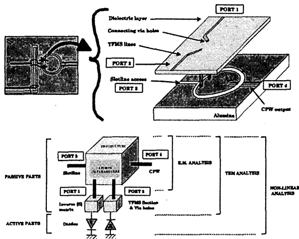
Fig. 7. Hybrid design procedure. Analysis: Procedure
