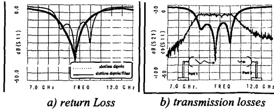
Fig. 2. Antenna-filter module – Characterization
