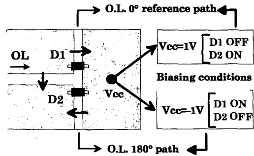
Fig. 4. magic TE in Modulator operating configuration
