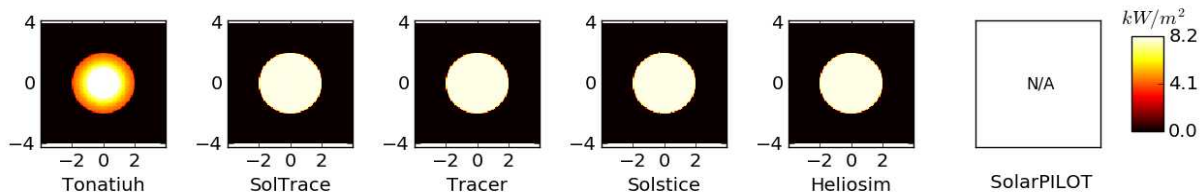
Fig. 4. Flux map of the 2 mrad pillbox slope error (Case A 1.1.2), the discrepancy of Tonatiuh shows the improper implementation of pillbox slope error. Flux map axis labels are in metres.
