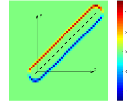
(c) \frac{\partial \delta}{\partial Y} , R = \frac{1}{2} dx , N_{gp} = 9
