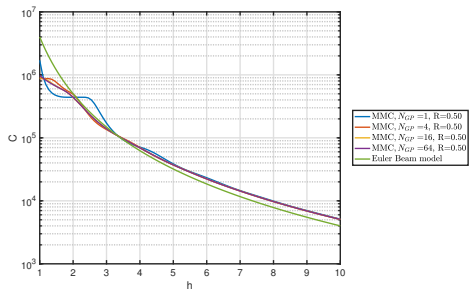
(a) h - C plot for R = 0.5 , N_{GP} = \{1, 4, 16, 64\}
