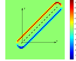
(b) \frac{\partial \delta}{\partial Y} , R = \frac{1}{2} dx , N_{gp} = 4
