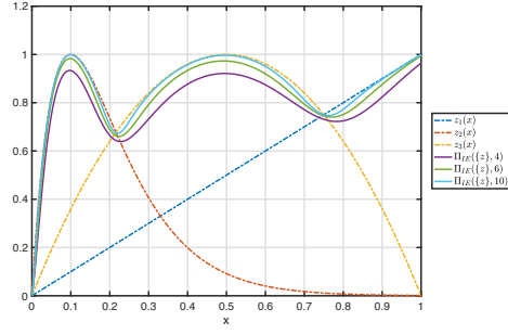
Fig. 13: Application of induced exponential aggregation function \Pi_{IE} for \kappa = 4, 6, 10 to the vector \mathbf{z} of 3 variables, z_1(x) = x , z_2(x) = 10xe^{1-10x} , z_3(x) = 4x(1-x) .
