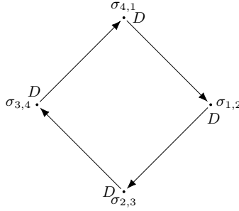
Fig. 4: The digraph of flips of G_4 and H_4 , where \sigma_{i,j} := (v_{i,1}v_{i,2}, v_{j,3}v_{j,4}) \rightarrow (v_{i,1}v_{j,3}, v_{i,2}v_{j,4}) for any i and j , and the label D stands for disconnected.
