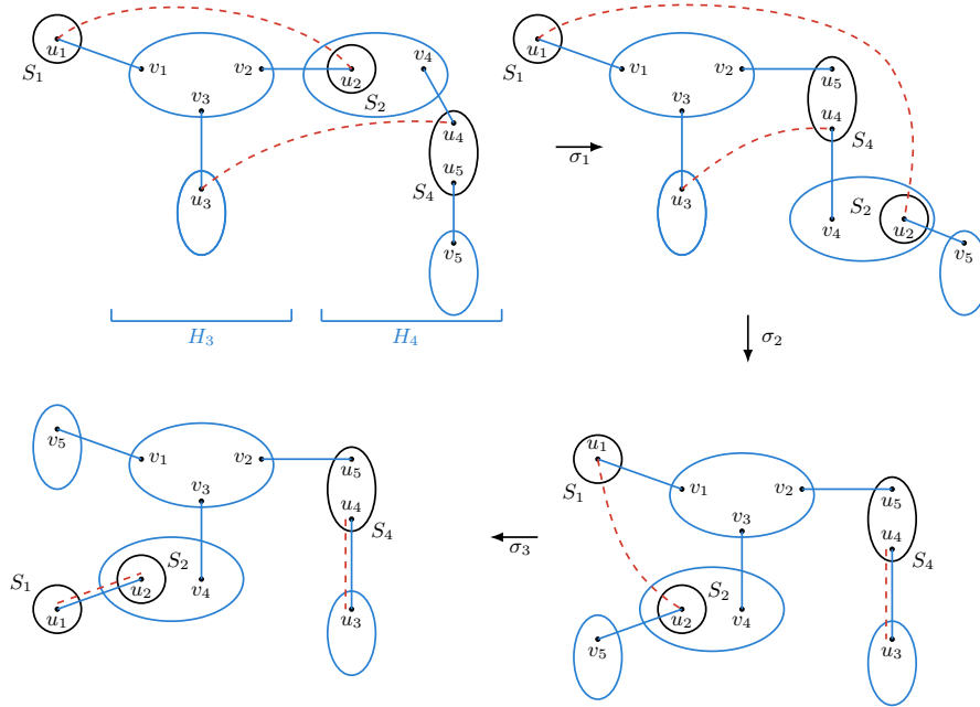
Fig. 2: The three flips \sigma_1 : (u_2v_2, u_5v_5) \rightarrow (u_2v_5, u_5v_2) , \sigma_2 : (u_3v_3, u_4v_4) \rightarrow (u_3u_4, v_3v_4) and \sigma_3 : (u_1v_1, u_2v_5) \rightarrow (u_1u_2, v_1v_5) applied to the graph H where (u_3, v_3, v_4, u_4) are aligned. The blue full edges are in E(H - G) and the red dashed edges are in E(G - H) .
