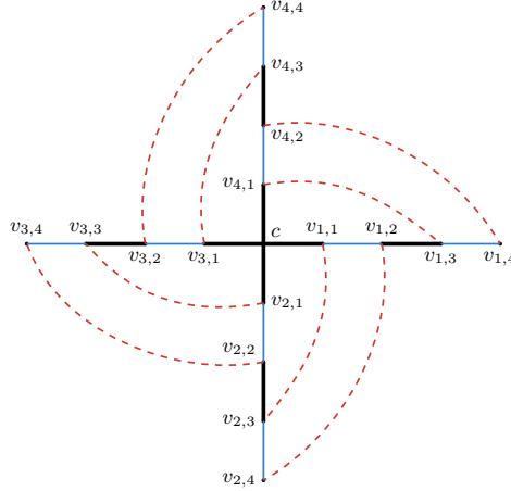
Fig. 3: The graphs G_4 and H_4 . The black thick edges are in E(G_4 \cap H_4) , the blue thin edges are in E(G_4 - H_4) and the red dashed edges are in E(H_4 - G_4) .
