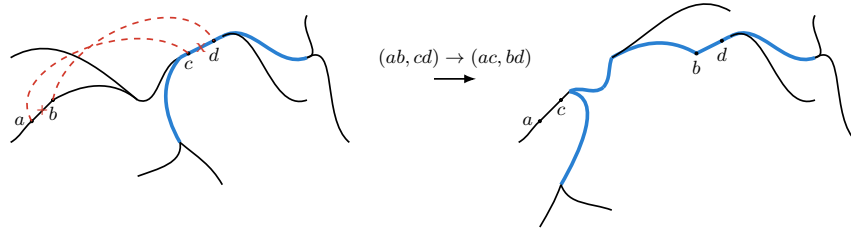
Fig. 1: The consequences of a connected flip in a tree. The blue thick path goes from an edge of the in-area of ab and cd to an edge of an out-area before the flip, and links the two same edges afterwards.
