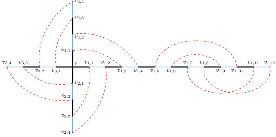
Fig. 5: G'_4 and H'_4 . The black thick edges are in E(G'_4 \cap H'_4) , the blue thin edges are in E(G'_4 - H'_4) and the red dashed edges are in E(H'_4 - G'_4) .
