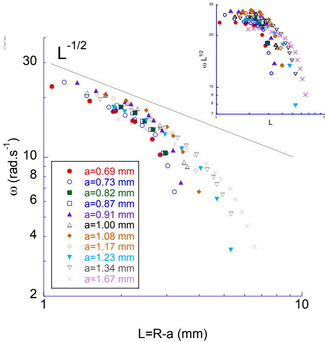
Fig. 4: Orbital speed of the drop \omega = d\theta/dt versus the orbit radius followed by the drop: L = R - a . A large range of drop radii is reported: 0.69 mm - 1.67 mm. Insert: the ratio \omega L^{1/2} versus L , that clearly saturates for low L . Error bars have the same order of magnitude as the symbols, consequently they are not shown here.
