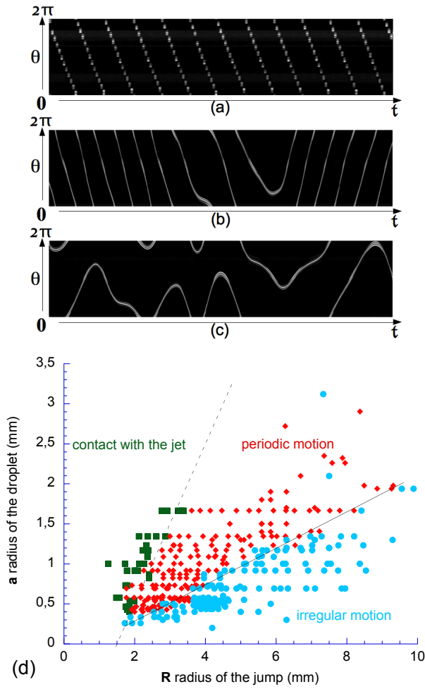
Fig. 2: Spatio-temporal diagrams obtained for a drop ( a = 1.1 mm) in the periodic regime (a) ( R = 4.6 mm and the recorded time is t_{tot} = 7.4 s) and in the irregular regime (b-c). Case (b) ( R = 5.5 mm and t_{tot} = 28.8 s) displays a single reversal of the sense of rotation just above the transition between periodic and irregular motion, while case (c) ( R = 5.9 mm and t_{tot} = 22.4 s) is obtained well above this one. (d) Phase diagram for the different kind of drop motions. ( \bullet ) irregular motion, ( \blacklozenge ) periodic motion and ( \blacksquare ) drop in contact with the jet
