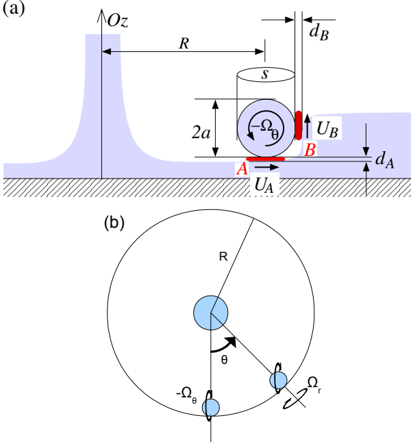
Fig. 3: (a) Notations and structure of the problem expected in a radial vertical plane containing the jump central axis. The drop is rotating very fast because of the shear stress transmitted across the air film. (b) Principle of the instability (top view). The drop tries to keep constant its kinetic momentum, which develops an active radial component of the rotation vector that tends to amplify the drop displacement.
