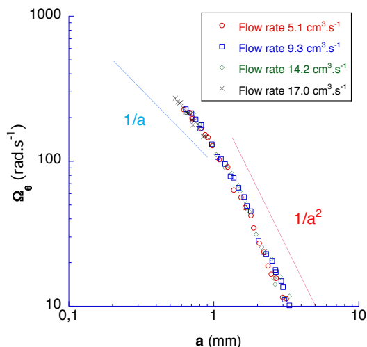
Fig. 6: \Omega_\theta versus drop radius observed for the stabilized inclined static case. Different flow rates are considered but all the curves are collapsing onto a single master curve without any rescaling, which suggests that the surface velocity at the jump could be the same for each flow rate. Error bars have the same order of magnitude as the symbols, consequently they are not shown here.
