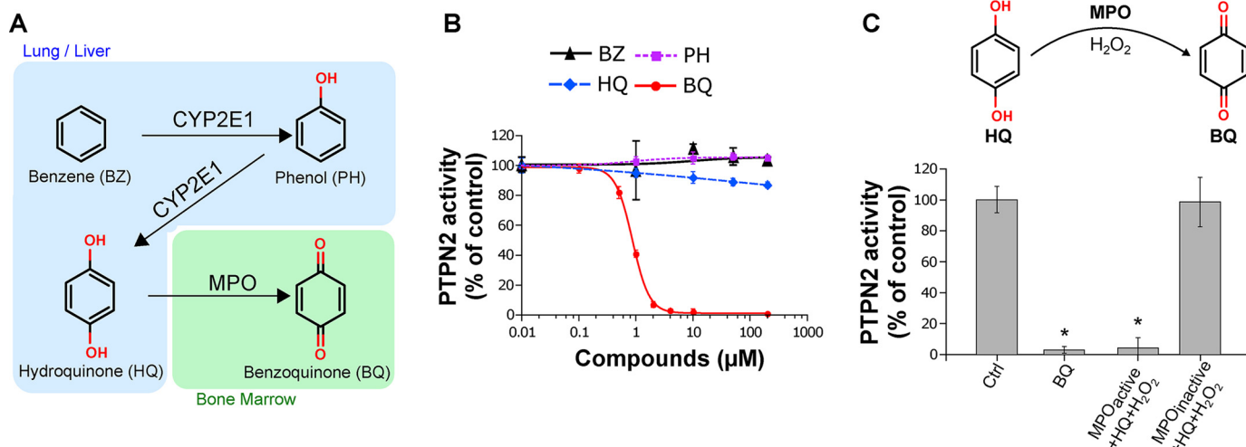
Figure 1. Effect of benzene and its metabolites on human PTPN2 activity. A , schematic representation of the benzene bioactivation pathway (1). B , human PTPN2 was incubated with increasing concentrations of benzene (BZ), phenol (PH), hydroquinone (HQ), or 1,4-benzoquinone (BQ) (0–200 \mu\text{M} ) for 20 min at 37 ^{\circ}\text{C} , and residual PTPN2 activity was measured using a pNPP assay. Error bars, S.D. values. C , human PTPN2 was incubated with or without BQ (10 \mu\text{M} ) or HQ in the presence of an active or inactive MPO hydroquinone-bioactivation system (including \text{H}_2\text{O}_2 ) for 20 min at 37 ^{\circ}\text{C} prior to residual PTPN2 activity assay. Error bars, S.D. *, p < 0.05 compared with control (Ctrl).
