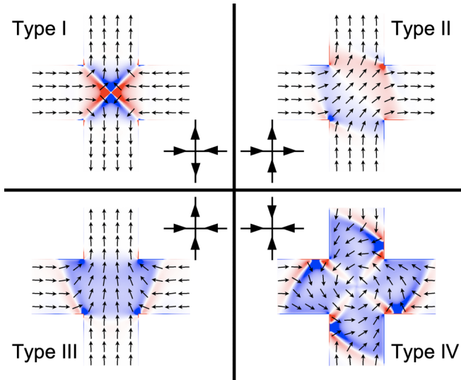
FIG. 2. Micromagnetic configurations of type-I, II, III, and IV vertices for 200-nm-wide, 20-nm-thick permalloy nanomagnets. Small black arrows represent the direction of magnetization within the nanomagnets, while the blue/red contrast codes for the divergence of the magnetization vector.
