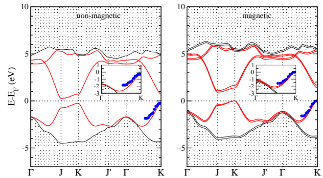
FIG. 5. The electronic band structure of the surface states of diamond C(111) 2 \times 1 surface, calculated with the HSE06 functional. Blue dots are the experimental ARPES data from Ref. 13. The ARPES data are shifted such that the valence band maximum of calculation and experiment match at the K-point.
