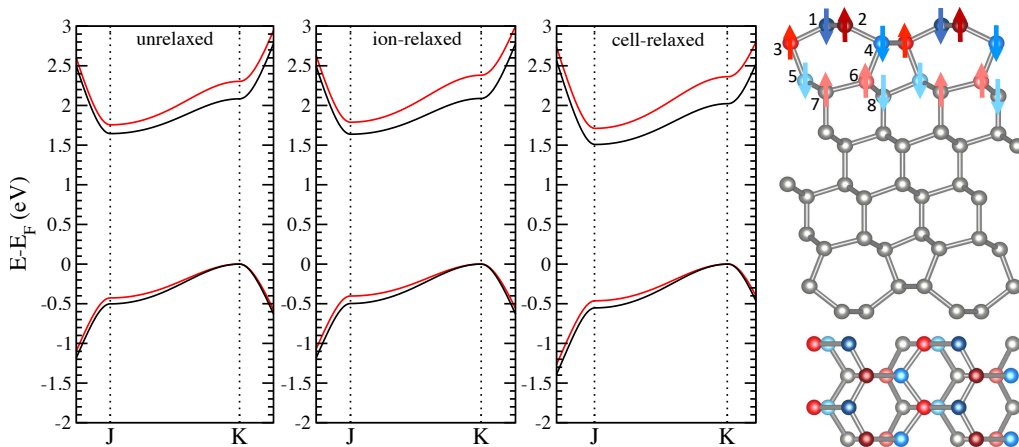
FIG. 3. Left: The effect of magnetism on the electronic structure of diamond C(111)2 \times 1 surface calculated with the PBE0 functional, with the unrelaxed (dimerized) structure of the non-magnetic calculation, and with the ion-relaxed and cell-relaxed calculations. Red is \alpha (majority) spin and black is the \beta (minority) spin electrons. Valence band maximum of each band is set to 0 eV. Right: The spin on each atom. Blue atoms are spin up and red atoms are spin down. The decrease in the shade of the color denotes the decrease in the magnitude of the atomic spin going towards the bulk. The arrows show the direction only and are not to scale. The magnitude of each spin is given in Table IV.
