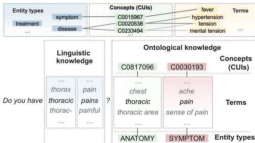
Fig. 7: Relation between entity types, concepts and terms. Linguistic knowledge processes affixes or morphological variants; ontological knowledge classifies terms into entity types; UMLS terms are indexed by Concept Unique Identifiers (CUIs)
