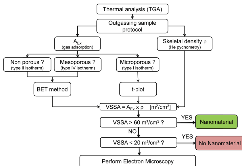
Fig. 1 Flow chart of the proposed operational powder characterization strategy for nanomaterial identification in the workplace.
