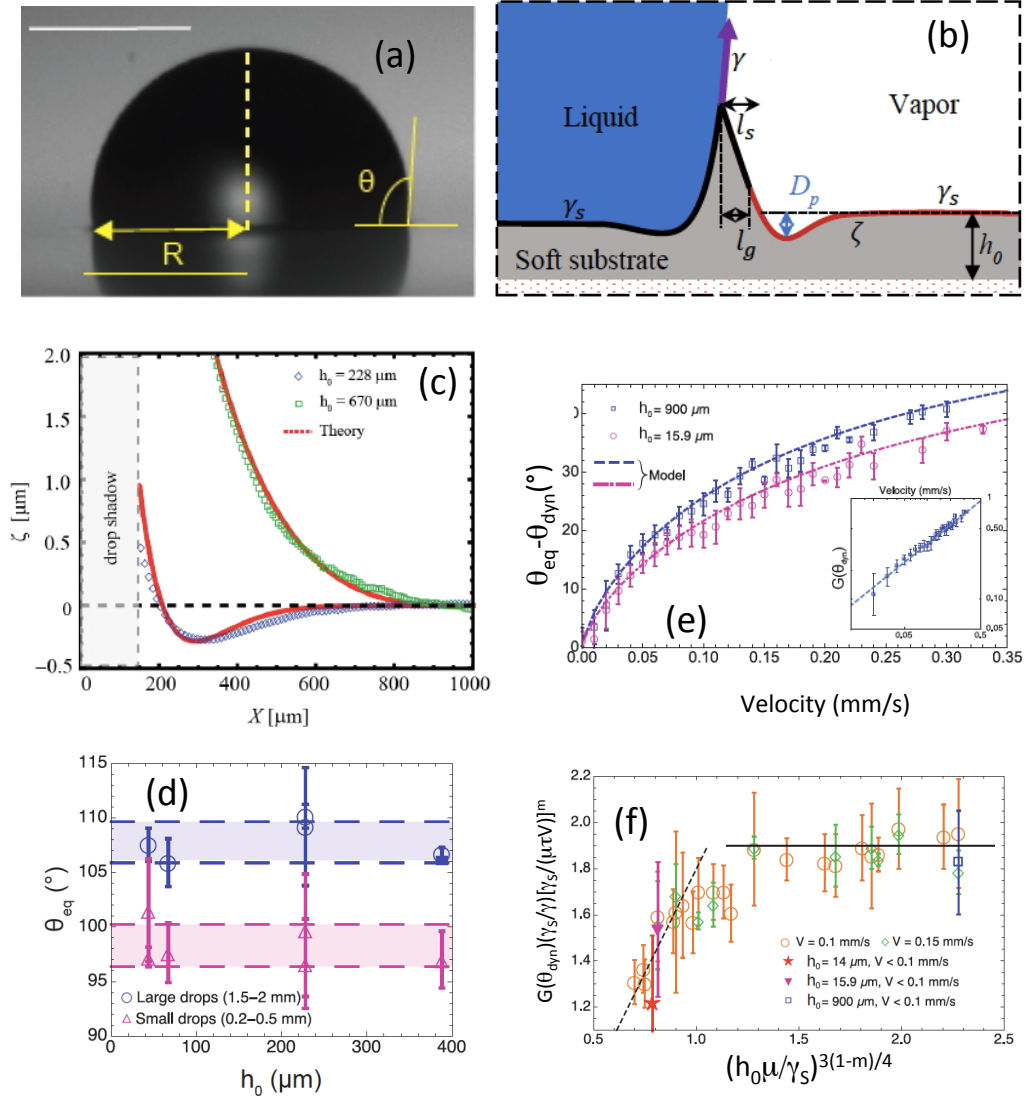
Figure 1: (a) side view of a drop deposited on the soft coating; (b) schematic of the details near contact line, (c) comparison of model and experimental profiles deduced from a Schlieren method; (d) static contact angles for “small” and “big” drops; (e) results obtained for the dynamical case, compared to modeling and, in the insert with the power law on the velocity deduced from eq. (3) ; (f) test with all data of our law (4), dotted line, while the law proposed in [3] is the continuous line.
