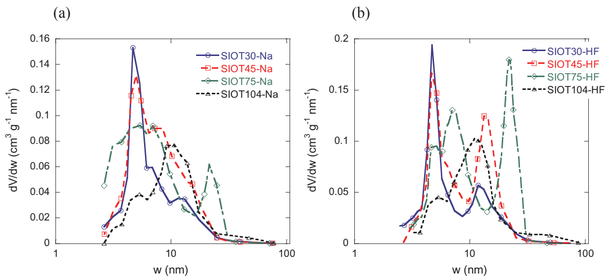
Fig. 6. Pore size distributions obtained by application of the BJH model to the desorption branches of \text{N}_2 isotherms for samples etched with: (a) NaOH, and (b) HF.
