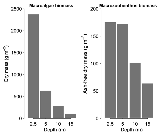
Fig. 2. Distributions of macroalgae (left panel) and macrozoobenthos (right panel) biomass along the depth gradient at Hansneset, Kongsfjorden, based on Bartsch et al. (2016) and Paar et al. (2016)
