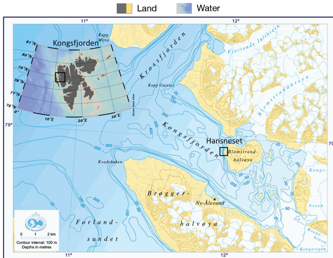
Fig. 1. Subtidal sampling site at Hansneset, west shore of Blomstrandhalvøya, in central Kongsfjorden (78°59.101'N, 11°57.793'E) in Spitsbergen (Svalbard archipelago, Norway). Overview maps were created with Ocean Data View (Schlitzer 2018). Map of Kongsfjorden was provided by the Norsk Polarinstitute
