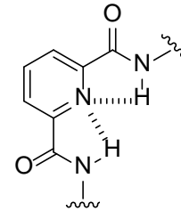
oligopyridine-2,6-dicarboxamides
