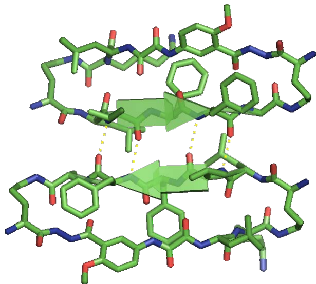
Anti-parallel \beta -sheet
