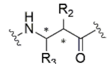
\beta^{2,3} -peptides
