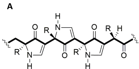
Oligopyrrolinones (Smith & Hirschmann)
