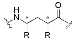
\gamma^{2,4} -peptides
