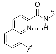
oligoquinolines
