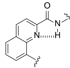
oligoquinolines
