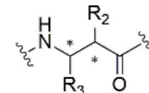
\beta^{2,3} -peptides
