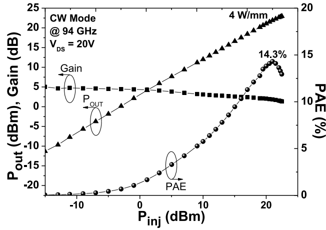
FIGURE 10. CW power performances of an AlN/GaN HEMT 2 \times 25 \mu\text{m} with L_G = 110 \text{ nm} for \text{GD} = 0.5 \mu\text{m} at V_{DS} = 20\text{V} .
