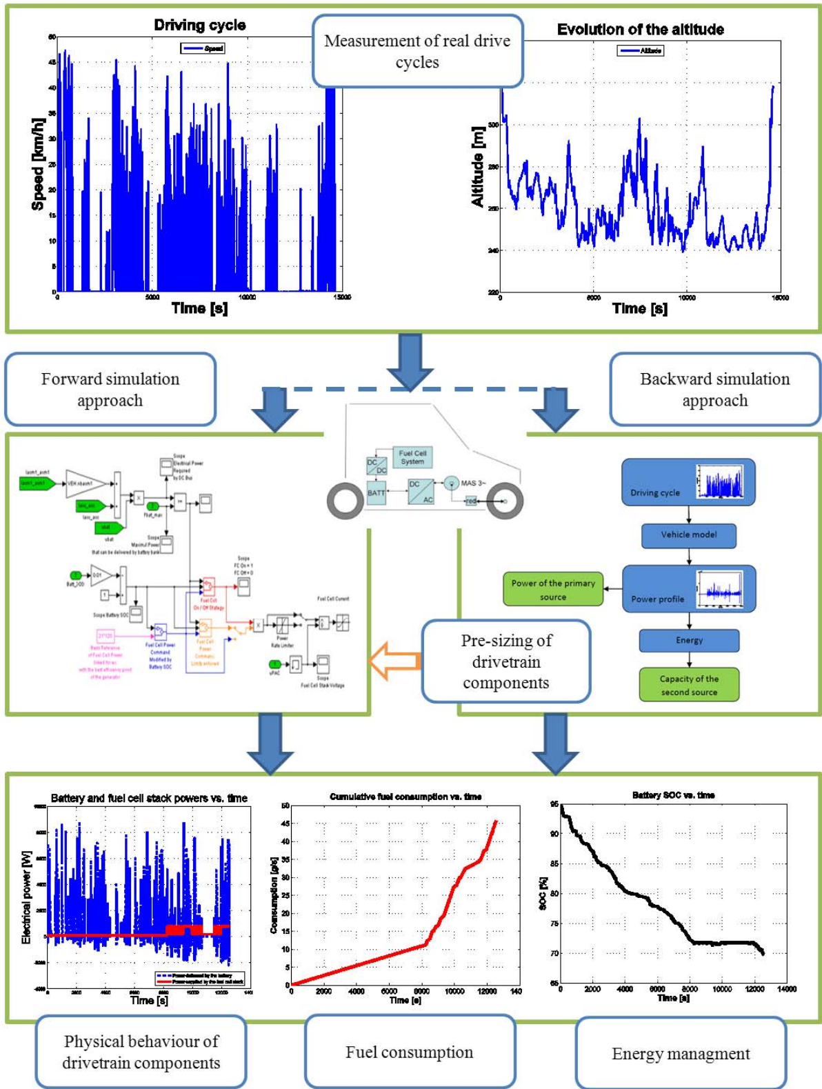
Figure 1: Methodology to design and simulate the MobyPost vehicle powertrain
