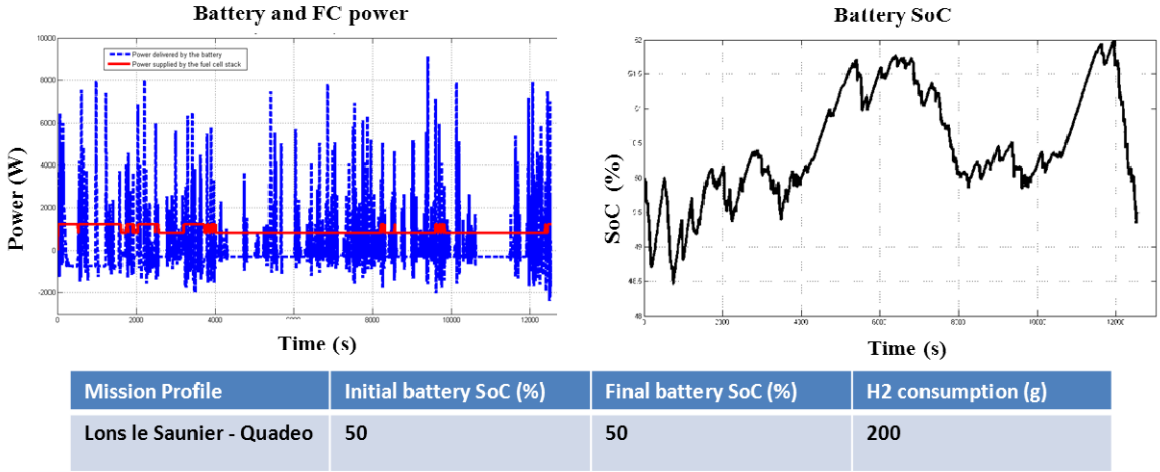
Figure 5: Simulation results with the forward approach of VEHLIB
