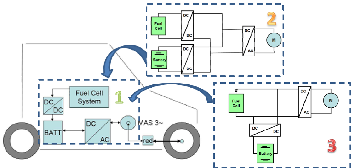
Figure 3: Electrical power train architectures
