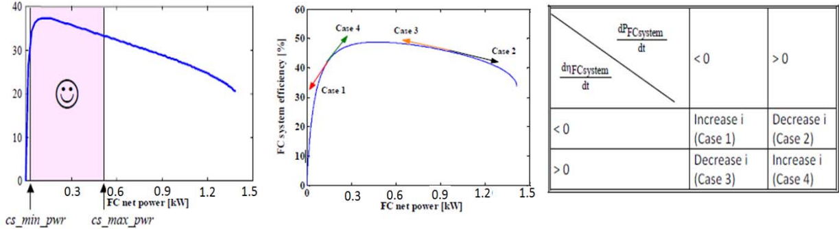
Figure 4: Fuel cell system efficiency [%] as a function of the net power [kW]
