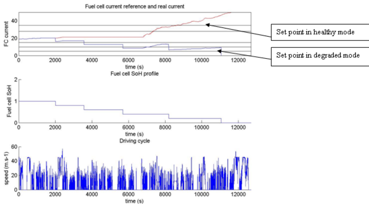
Figure 8: Dynamical simulation of the vehicle drivetrain on the Lons Le Saunier cycle with a fuel cell SoH variation
