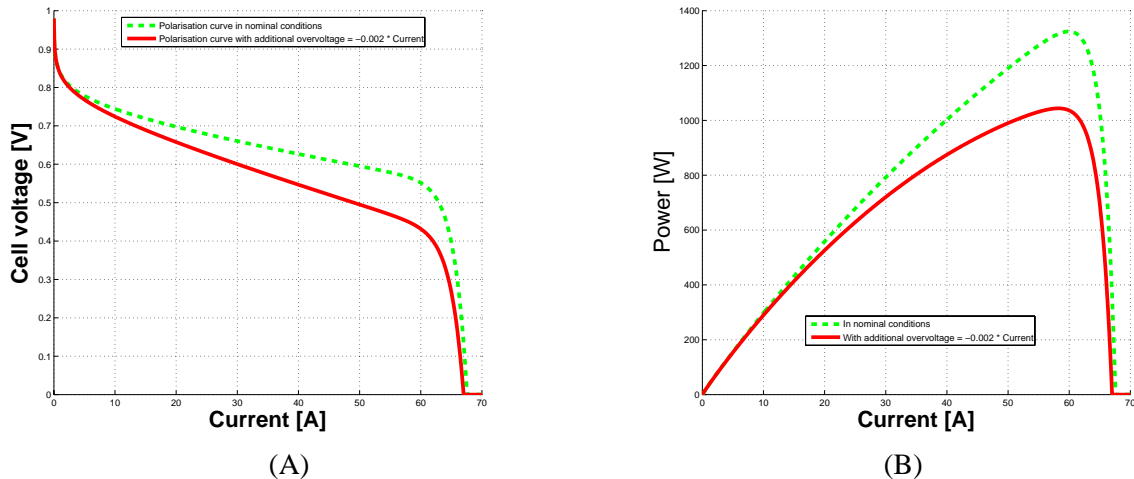
Figure 7: Comparison between the normal / nominal cell polarisation curve (healthy state) and the adopted fuel cell current– voltage curve representing the degraded individual cell performances (A). Comparisons in terms of stack power delivery (B).
