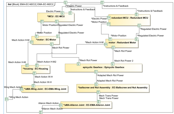
Fig. 10. EMA system physical architecture (variant 2).
