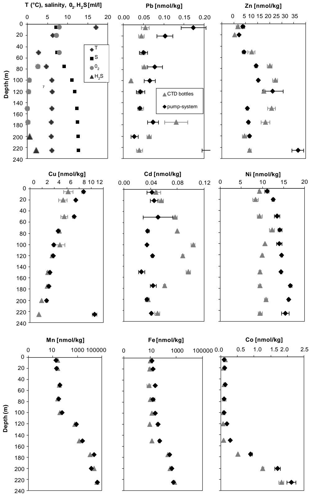
Fig. 4. Separated profiles, bottom to surface from July 2005: (a) profile of T (temperature, °C), S (salinity), dissolved oxygen and hydrogen sulphide (m/l) over depth and (b)–(i) profiles of dissolved Pb, Zn, Cu, Cd, Ni, Mn, Fe and Co (nmol/kg) sampled from the bottles and the Pump–CTD-System over depth.
