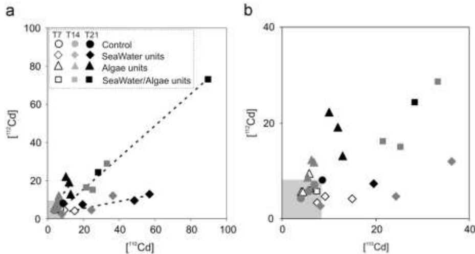
Fig. 6. (a) Mean [^{110}\text{Cd}] concentration (direct contamination) over mean [^{112}\text{Cd}] concentration (trophic contamination) measured in digestive glands of oysters from Control, SeaWater unit, Algae units and SeaWater/Algae units after 7, 14 and 21 days of experiment. (b) Zoom of (a). The grey area represents the natural variation content of [^{110}\text{Cd}] and [^{112}\text{Cd}] in oysters from Control.
