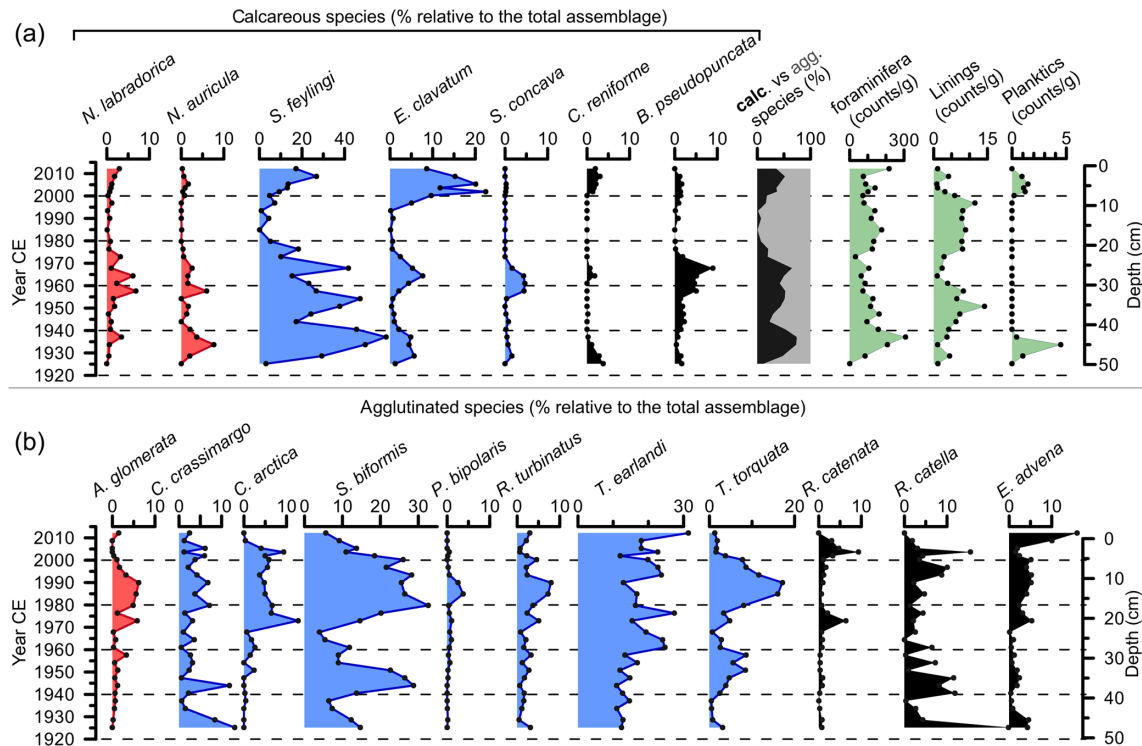
Figure 5. Abundances of calcareous (a) and agglutinated benthic foraminiferal species (b), plotted vs. age and depth in core POR13-05. Abundances are calculated relative to the total (calcareous and agglutinated) counts of benthic foraminifera. Red colours indicate (chilled) Atlantic water indicator species, blue colours represent water indicators. Only species representing > 0.5\% of the total assemblage are shown. Total count of foraminifera and organic linings per gram are also indicated (green, a). Stippled lines are a visual aid for comparing the different trends.
