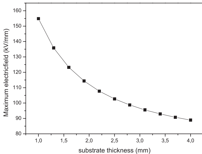
Fig. 9. Maximum electric field at the triple point as a function of substrate thickness for the conventional structure.
