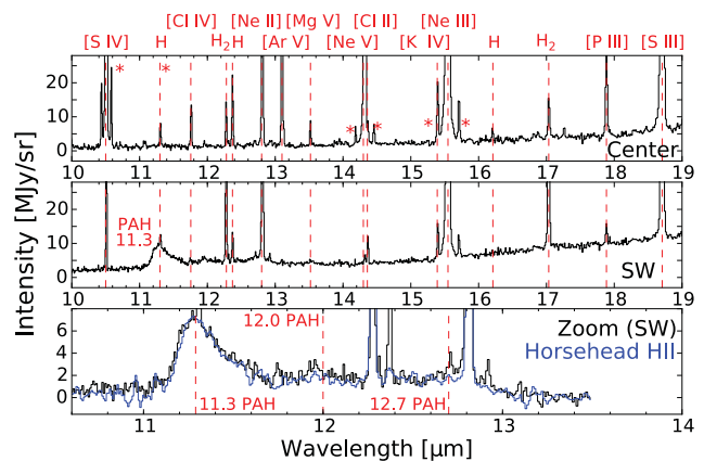
Figure 2. Spitzer –IRS SH spectra extracted from the 3D spectral-cube at two positions in the Ring Nebula. The positions are indicated by the two white-dashed squares in Fig. 1. The top panel shows a spectrum from the central hot-gas cavity and the middle panel shows the spectrum ‘SW’ arising from the main dust ring. Emission lines arising from several atoms and molecular hydrogen are labelled (ghost lines are indicated with asterisks). The bottom panel shows a close-up view of the (continuum subtracted) 11–13 \mu\text{m} PAH emission complex. The PAH emission spectrum of the Horsehead H II region (Compiègne et al. 2007), scaled by a factor of 0.4 to match the 11.3 \mu\text{m} peak intensity, is shown for reference.
