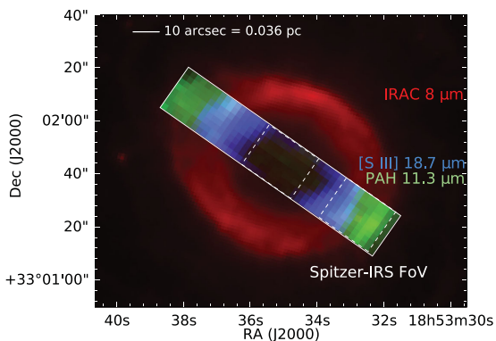
Figure 1. Spitzer –IRS maps of the 11.3 \mu\text{m} emission feature (green) and the [S III] emission line (blue) in the Ring Nebula overlaid on top of the Spitzer IRAC 8 \mu\text{m} image (red). The two white squares (dashed lines) indicate the extraction region for the spectra shown in Fig. 2.
