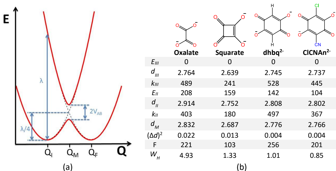
Figure 9. (a) Energy plot for a Fe^{II}Fe^{III} to Fe^{III}Fe^{II} electron transfer process. (b) Calculated parameters for the four studied bridging ligands. Distances are expressed in Å, energies in kcal.mol^{-1} , k and F in kcal.mol^{-1}.\text{Å}^{-2} .
