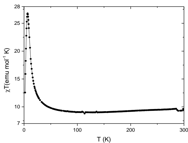
42 43 44 45 46 47 48 49 50 51 52 53 54 55 56 57 58 59 60 Figure 3. Temperature dependence of the product of the molar magnetic susceptibility times the temperature ( \chi_m T ) of 1 under an applied field of 1000 Oe.
