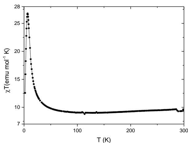
41 42 43 44 45 46 47 48 49 50 51 52 53 54 55 56 57 58 59 60 Figure 3. Temperature dependence of the product of the molar magnetic susceptibility times the temperature ( \chi_m T ) of 1 under an applied field of 1000 Oe.
