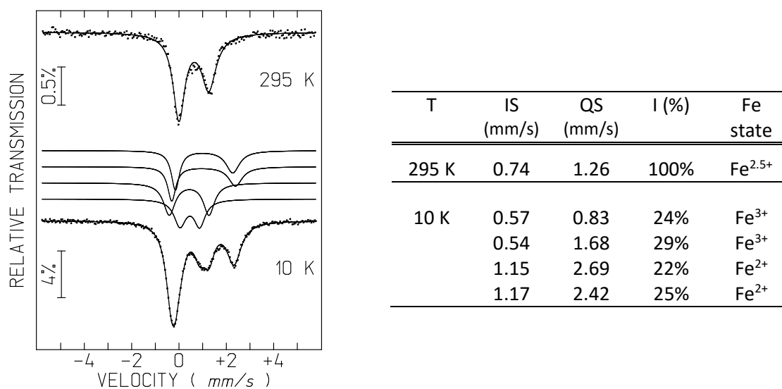
Figure 6. (a) Mössbauer spectra of 1 taken at 295 and 10 K and (b) estimated parameters from the spectra. The lines over the experimental points are the calculated functions. On the spectrum taken at 10 K this function is the sum of four quadrupole doublets shown slightly shifted for clarity. IS, isomer shift relative to metallic \alpha -Fe at 295 K; QS, quadrupole splitting; I, relative areas. Estimated errors are < 0.02 mm/s for IS, QS, < 2\% for I.
