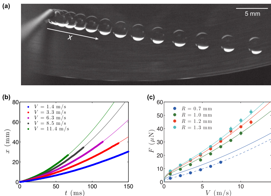
FIG. 3. Estimating aerodynamic forces from drop acceleration. (a) Chronophotograph of a drop of silicone oil ( R = 1.25 mm) deposited at 1 cm from the edge of a plate rotating at V = 3.5 m/s. Successive images are separated by 12.5 ms. The drop is entrained along a quasistraight line and its position is denoted by x . (See movies 5 and 6 in Ref. [22].) (b) Position x as a function of time t for various plate velocities V . Thin lines are parabolic fits x = at^2 , from which we deduce a constant force of entrainment F = 2ma . (c) Force F as a function of plate velocity V , for various drop radii R . Lines show Eq. (2) drawn with \alpha = 3 and \beta = 0.55 . The dotted line is the best fit ( \alpha = 1.7 and \beta = 0.55 ) for the smallest droplet of radius R = 0.7 mm.
