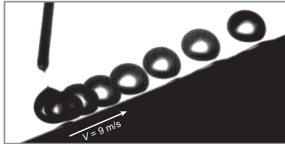
FIG. 4. Chronophotograph of a drop of silicone oil ( R = 0.94 \text{ mm} ) dispensed by a needle (on the left) on a surface inclined by an angle of 22^\circ and moving to the right at V = 9 \text{ m/s} . The aerodynamic entrainment force F is large enough to push oil up and accelerate it against gravity. Successive images are separated by 8 ms.
