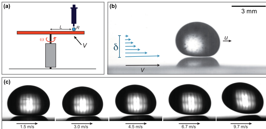
FIG. 1. Aerodynamic Leidenfrost effect. (a) Schematic of the experimental setup. A drop of viscosity \eta = 96 mPa s and millimeter-size radius R is gently deposited from a syringe on a disk of aluminum rotating at an angular velocity \omega . The disk velocity under the drop is denoted by V . (b) Side view of a drop of silicone oil (with R = 1.24 mm) for \omega = 44 rad/s and V = 4 m/s (see movie 1 in Ref. [22]). Levitation is observed, as shown by the nonwetting shape of the drop and by the ray of light between the liquid and its reflection. The disk entrains a boundary layer of thickness \delta \approx 2.5(\eta_a/\rho_a\omega)^{1/2} \approx 1.5 mm, whose profile is sketched in blue, at the correct scale. Due to the plate motion, the drop drifts at a velocity u \ll V . (c) As the plate velocity V increases from 1.5 m/s to 9.7 m/s, the gap thickness also increases (see movies 2–4 in Ref. [22]). Here the drop size is kept constant with R = 1.24 mm.
