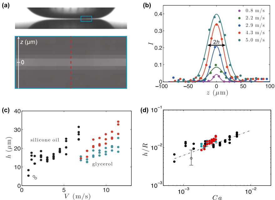
FIG. 2. Measurements of air gap thickness. (a) Base of a drop of silicone oil ( R = 1.24 mm) levitating above an aluminum plate moving from left to right at V = 3.0 m/s. The thickness of air is measured in the flat zone where it is minimum (blue box). In this area, the gray shade of each pixel is measured along the dashed vertical line as a function of the position z . (b) Variations of the pixel intensity I as a function of z , for five surface velocities V . Circles show data and lines are Gaussian fits, whose width provides the thickness h . (c) Air thickness h as a function of plate velocity V . Black and blue data points correspond to silicone oil and glycerol of radius R = 1.24 mm and red data points correspond to bigger drops of glycerol ( R = 1.68 mm). Open symbols indicate measurements by Lhuissier et al. [14], performed by colored interferometry through a transparent substrate (for R = 1.16 and 1.39 mm). (d) A log-log plot of the ratio h/R as a function of the capillary number Ca = \eta_a V / \gamma , with \eta_a the air viscosity and \gamma the surface tension of the drop. The open symbol summarizes all the data by Lhuissier et al. [14], obtained at a velocity V = 1.54 \pm 0.11 m/s and R = 0.55, 1.16, 1.39 mm. The data collapse and they are consistent with the power law h = 0.60 R Ca^{2/3} represented by a dotted line.
