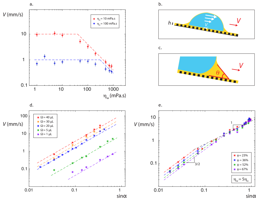
Figure 2. (a) Speed V of a descending drop ( \Omega = 20 \mu\text{L} ) as a function of its viscosity \eta_w , at fixed oil viscosity ( \eta_o = 10 \text{ mPa}\cdot\text{s} , red data; \eta_o = 100 \text{ mPa}\cdot\text{s} , blue data), on a substrate with \phi = 23\% tilted by \alpha = 5^\circ . Two regimes are successively obeyed: for \eta_w < \eta_o , V is independent of \eta_w ; for \eta_w > \eta_o , V becomes inversely proportional to \eta_w (inclined lines have a slope -1 ). Both regimes intersect at a critical water viscosity \eta_w^* \approx 3\eta_o . (b) Sketch of a viscous drop going down a lubricant-impregnated surface, for which the Poiseuille flow within the drop limits the speed. We denote as V_i the velocity of the water/oil interface. (c) The front of the moving meniscus is dynamically deformed, with an angle \theta(V) . (d) Speed V of descending drops with viscosity \eta_w = 2 \text{ mPa}\cdot\text{s} and \Omega = 1 \mu\text{L} (purple data), \Omega = 5 \mu\text{L} (green data), \Omega = 20 \mu\text{L} (blue data), \Omega = 30 \mu\text{L} (orange data), \Omega = 40 \mu\text{L} (red data). The surface ( \phi = 23\% ) is impregnated by oil with viscosity \eta_o = 100 \text{ mPa}\cdot\text{s} . (e) Speed V of a descending drop ( \eta_w = 500 \text{ mPa}\cdot\text{s} ) on a surface impregnated with oil of comparable viscosity ( \eta_o = 100 \text{ mPa}\cdot\text{s} ). Two regimes are successively observed, with power laws of respective exponent 3/2 and 1 . Both regimes intersect at a critical speed V^* \approx 2 \text{ mm/s} .
