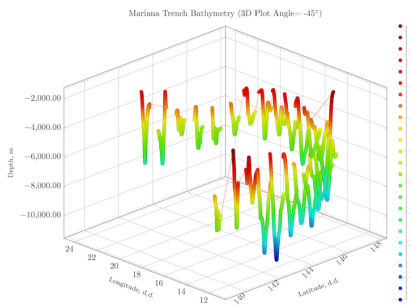
Mariana Trench Bathymetric Profiles. 3D Plotting: L A T E X
