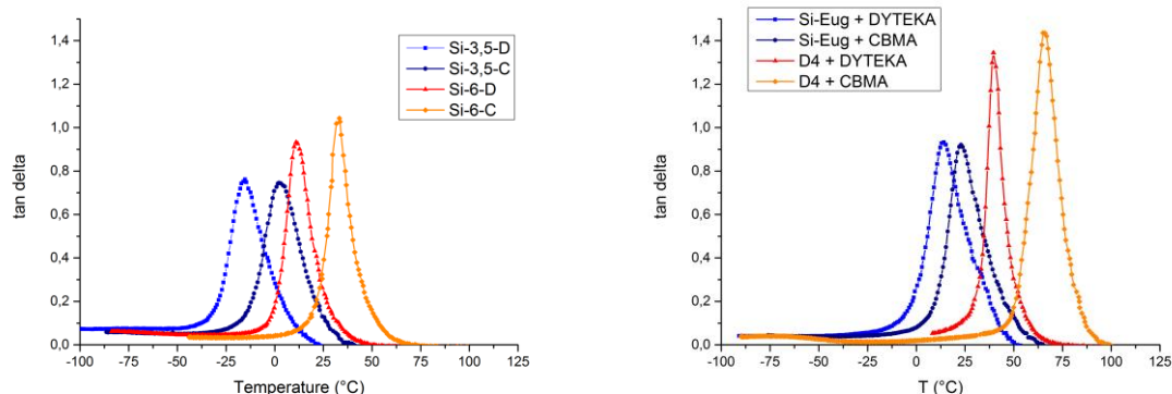
Figure 9. Tan delta versus temperature of PHU thermosets (left: Si-3.5 and Si-6; right: Si-Eugenol and D4)
