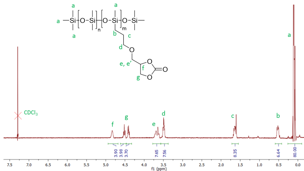
Figure 3. ^1\text{H-NMR} ( \text{CDCl}_3 ) spectrum of Si-3.5 carbonate monomer
