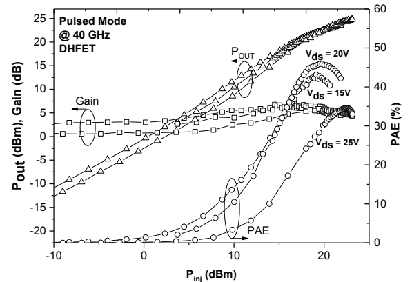
Fig. 4.2. : Pulsed power performance of a 0.12 \times 50 \mu\text{m}^2 DHFET at 40 GHz with V_{DS} = 15, 20, 25\text{V} .
