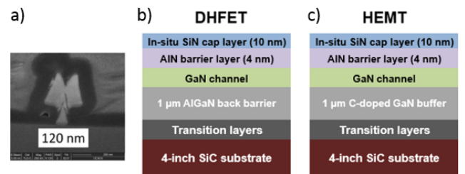
Fig. 2.1. : a) FIB view of the 0.12 \mu m T-gate and schematic cross section of b) DHFET and c) C-doped HEMT.
