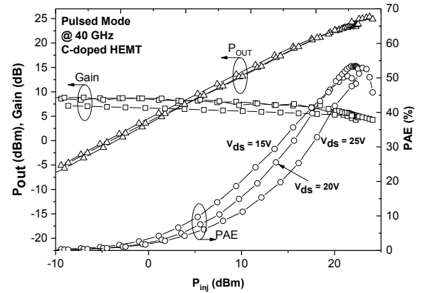
Fig. 4.1. : Pulsed power performance of a 0.12 \times 50 \mu\text{m}^2 HEMT at 40 GHz with V_{DS} = 15, 20, 25\text{V} .
