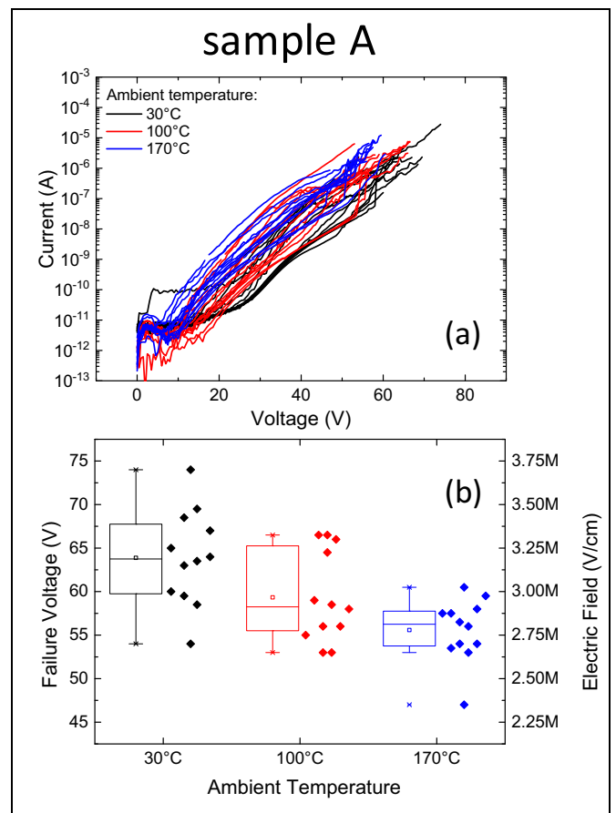
Fig. 3. (a) Current-voltage characteristics of the devices on sample A at different ambient temperature (i.e. 30 °C, 100 °C and 170 °C). (b) Box chart of the failure voltages of the tested device of sample A. Right y-axis shows the corresponding electric field.
