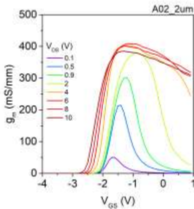
Fig - 1. g_m versus V_{GS} characteristics of a representative AlN/GaN HEMT
