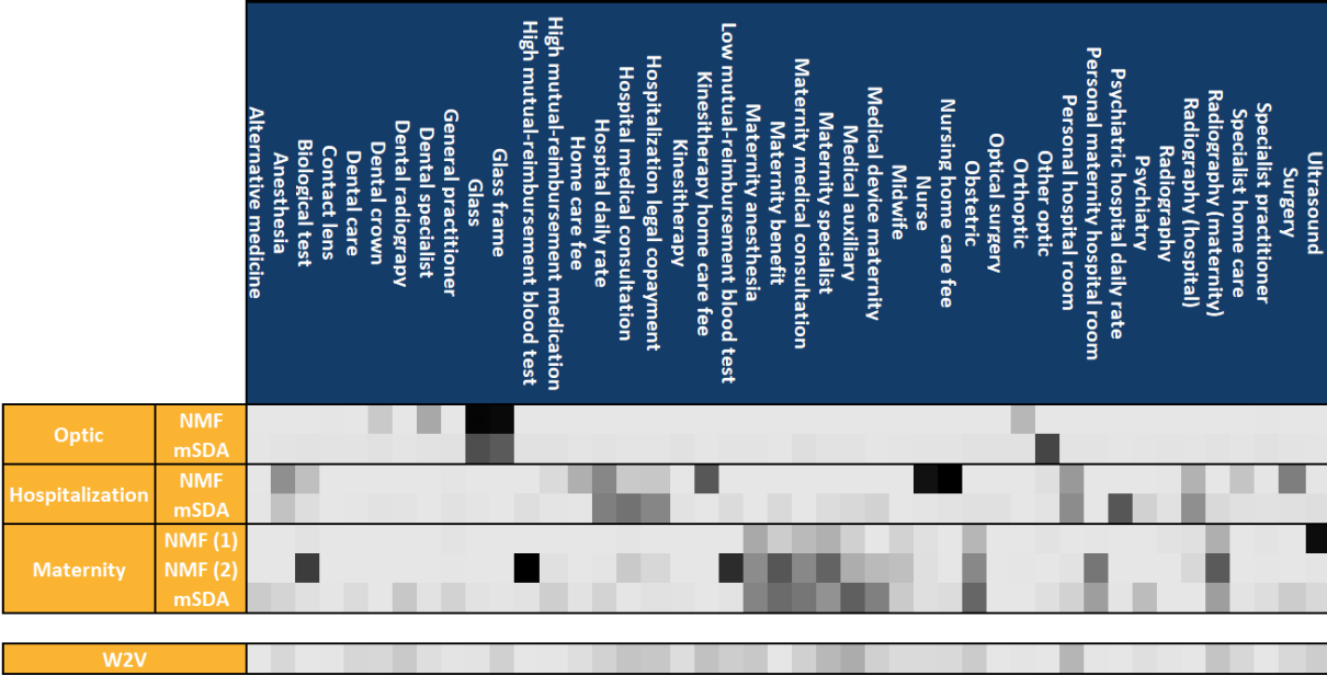
Figure 3: Dimension reduction leads to Medical Act Clusters. The last line is a vector of the embedding offered by W2V, illustrating that this embedding is not meaningful. NMF(1) and NMF(2) are two medical act classes produced by the NMF method and probably linked to maternity.
