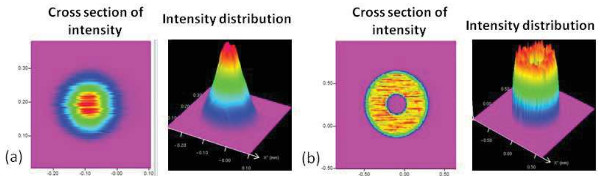
Figure 2: Intensity distributions at the focal point with (a) the 100 \mu\text{m} core fiber (500 W, \Phi=150 \mu\text{m} ), (b) the 400 \mu\text{m} outer fiber (500 W, \Phi=150 \mu\text{m} ) measured with a Primes Focus monitor device.
