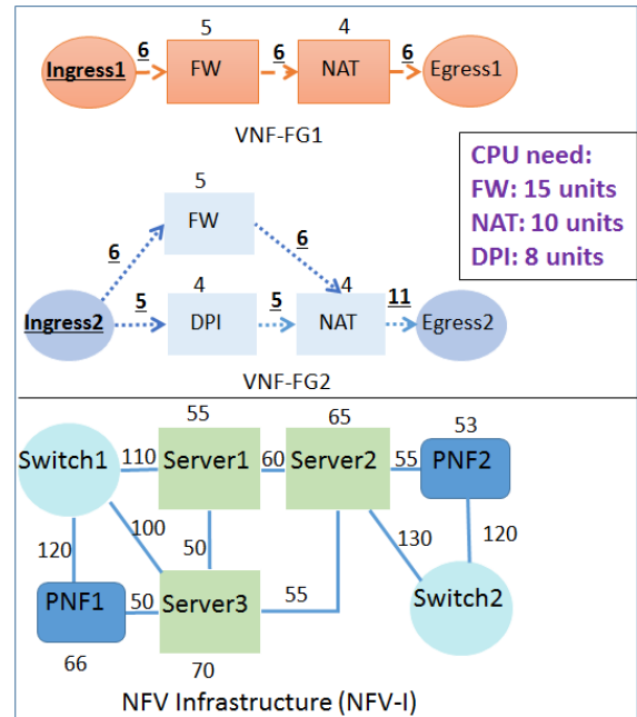
Figure 1: An example of SFC and NFV-I topologies
