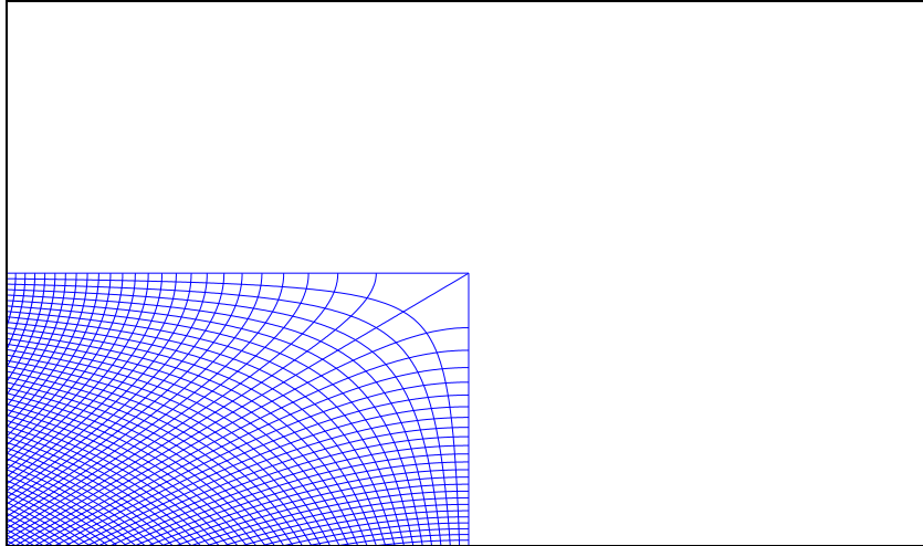
FIGURE 3. The image of \Psi(z) = -2z^{1/2}
