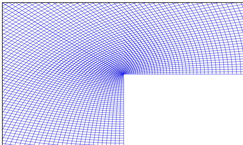
FIGURE 2. The image of \Psi(z) = \frac{2}{3}z^{3/2}
