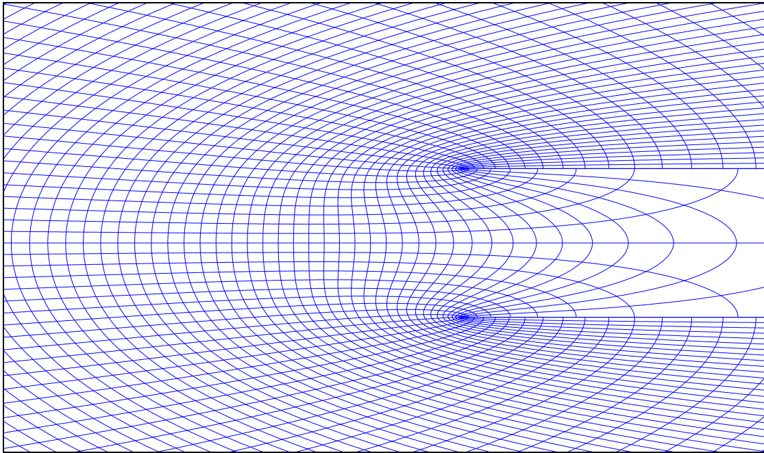
FIGURE 1. The image of \Psi(z) = z^2/2 - \log(z)
