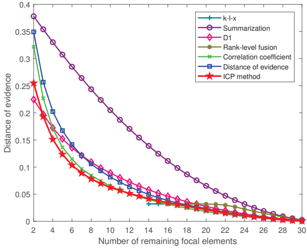
Fig. 3. Closeness comparisons.
