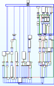
Figure 1: Control-flow graph of a quick-sort function obfuscated using several Tigress transformations.
