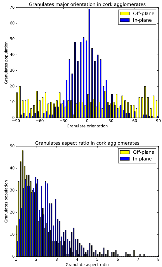
Fig. 5. Results of picture analysis. Histograms of the granulates orientation and of their aspect ratio.
