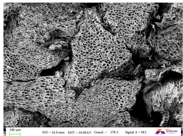
Fig. 6. Random cells orientation in cork agglomerates.
