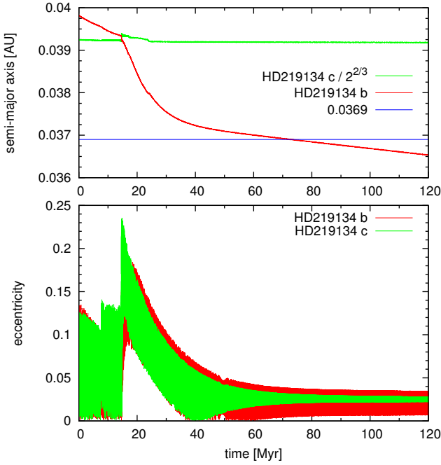
Fig. 6: Evolution of the inner two planets of the HD219134 system under dissipation with k_2/Q = 0.025 for both planets, and in presence of planets f and d of Gillon et al. (2017). Top panel: semi-major axis of planet b (red curve), location of the 1:2 mean motion resonance with planet c (green curve, that is a_c/2^{2/3} ), and present semi-major axis of planet b (blue horizontal line). Bottom panel: eccentricities of planets b (red) and c (green).
