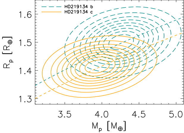
Fig. 4: Joint likelihood of the planetary mass and radius for planet b (green long-dashed line) and planet c (yellow solid line). The 9 contour lines separate 10 equal-sized intervals between 0 and the maximum of f_p(M_p, R_p) . The dashed lines show the iso-densities corresponding to the mean densities of planets b and c .
