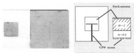
a - Patch antenna with a CPW feeder on a composite foam/ceramic substrate
