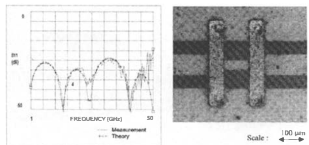
FIG. 7. — B-type compensation.
