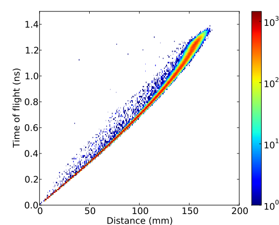
Fig. 4: Time of \gamma creation as a function of distance from hodoscope.
