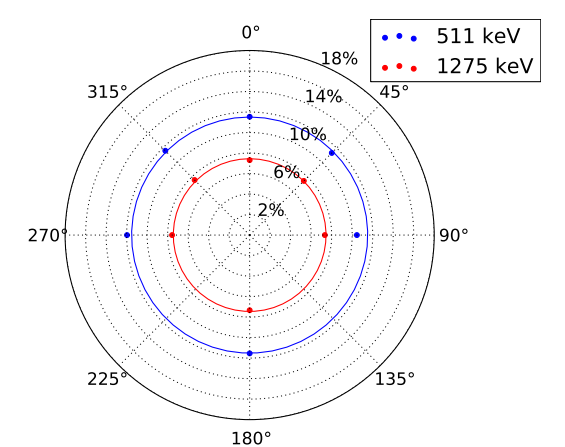
Fig. 7: Energy resolution as a function of angle.
