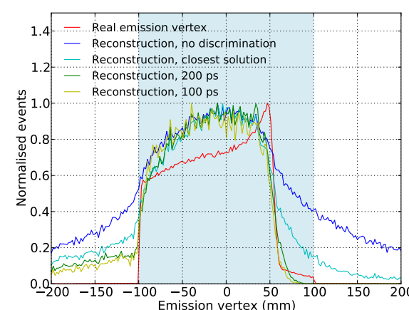
Fig. 6: The real \gamma emission vertex along the beam axis compared to reconstructions with different criteria.
